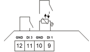
JOY Fancoil EC 3AO (24 V ~/=)
