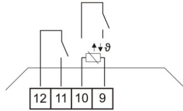
JOY Fancoil EC AO2DO (85..260 V ~)
