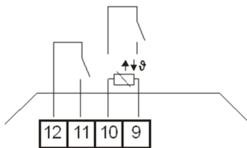
JOY Fancoil 5DO (85..260 V ~)
